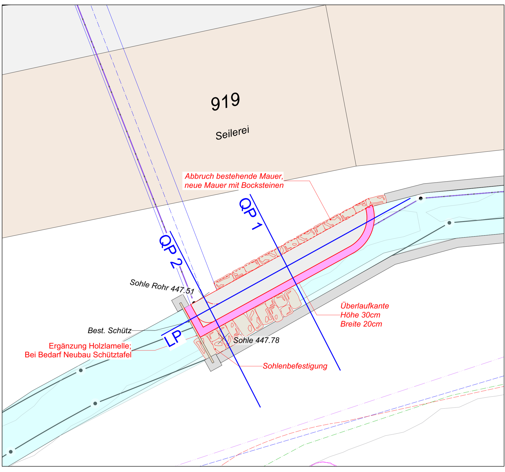
Detailplan, M 1:50
