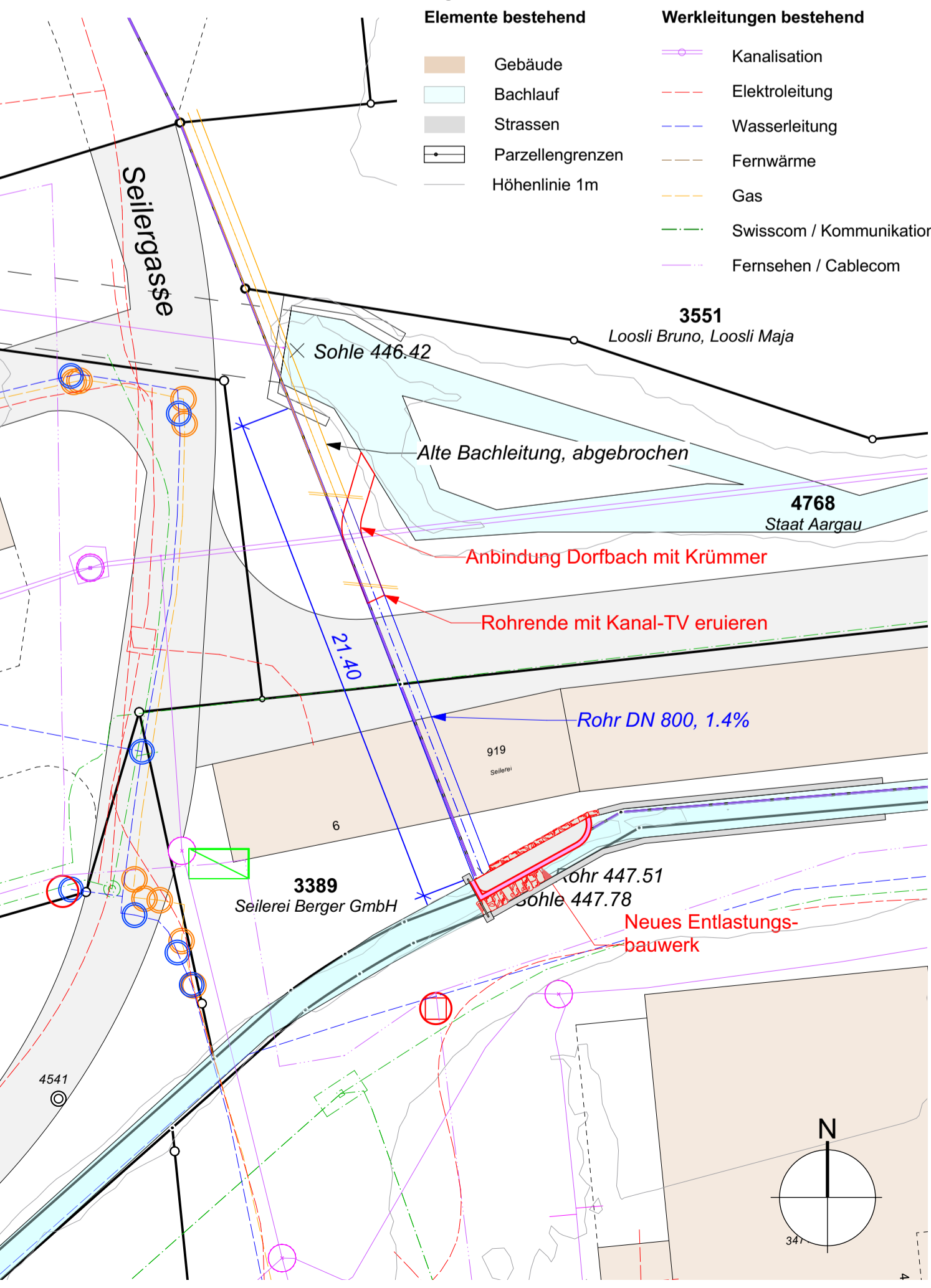
Situation, M 1:200
